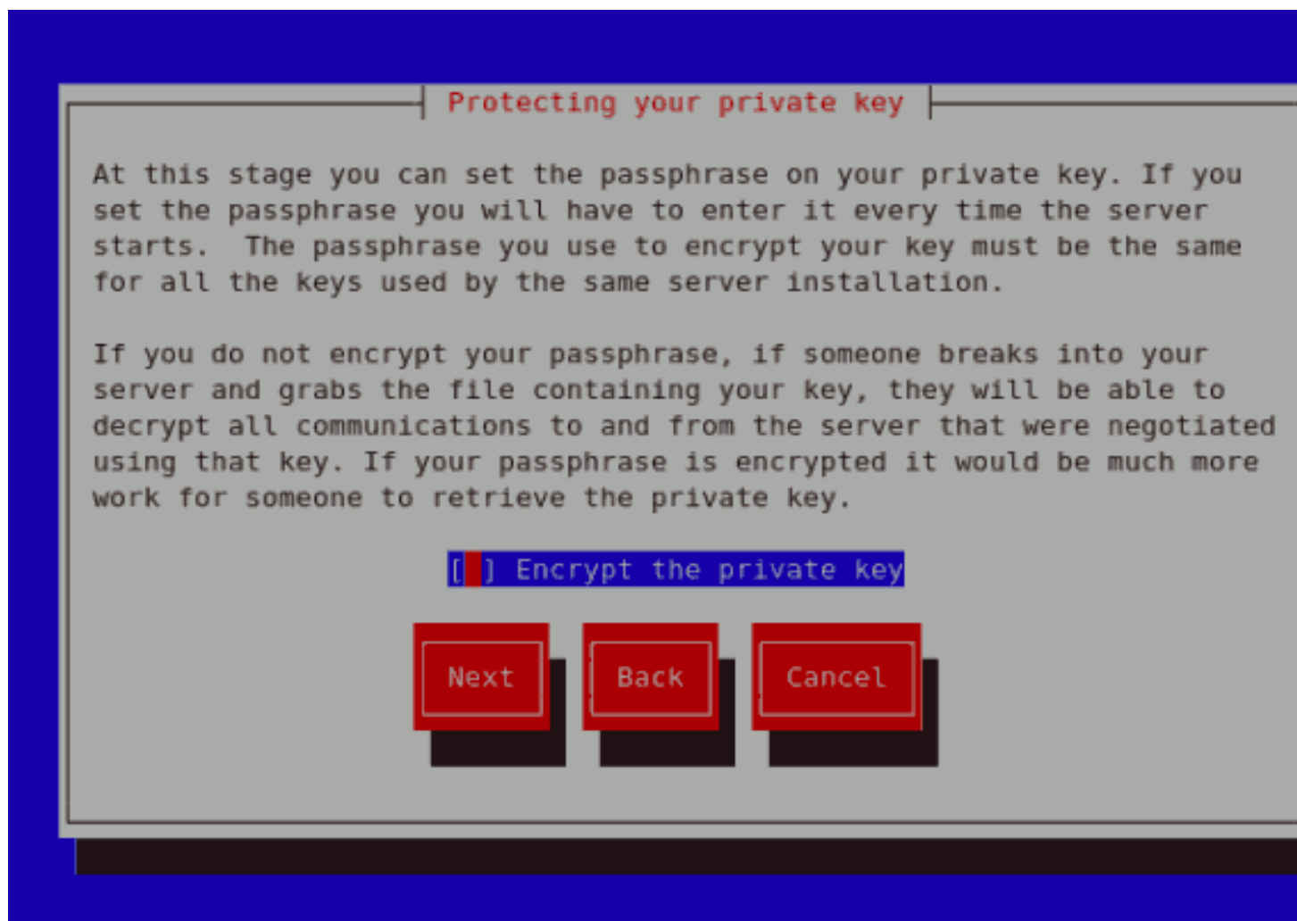
Figure 23.19. Protecting your private key
