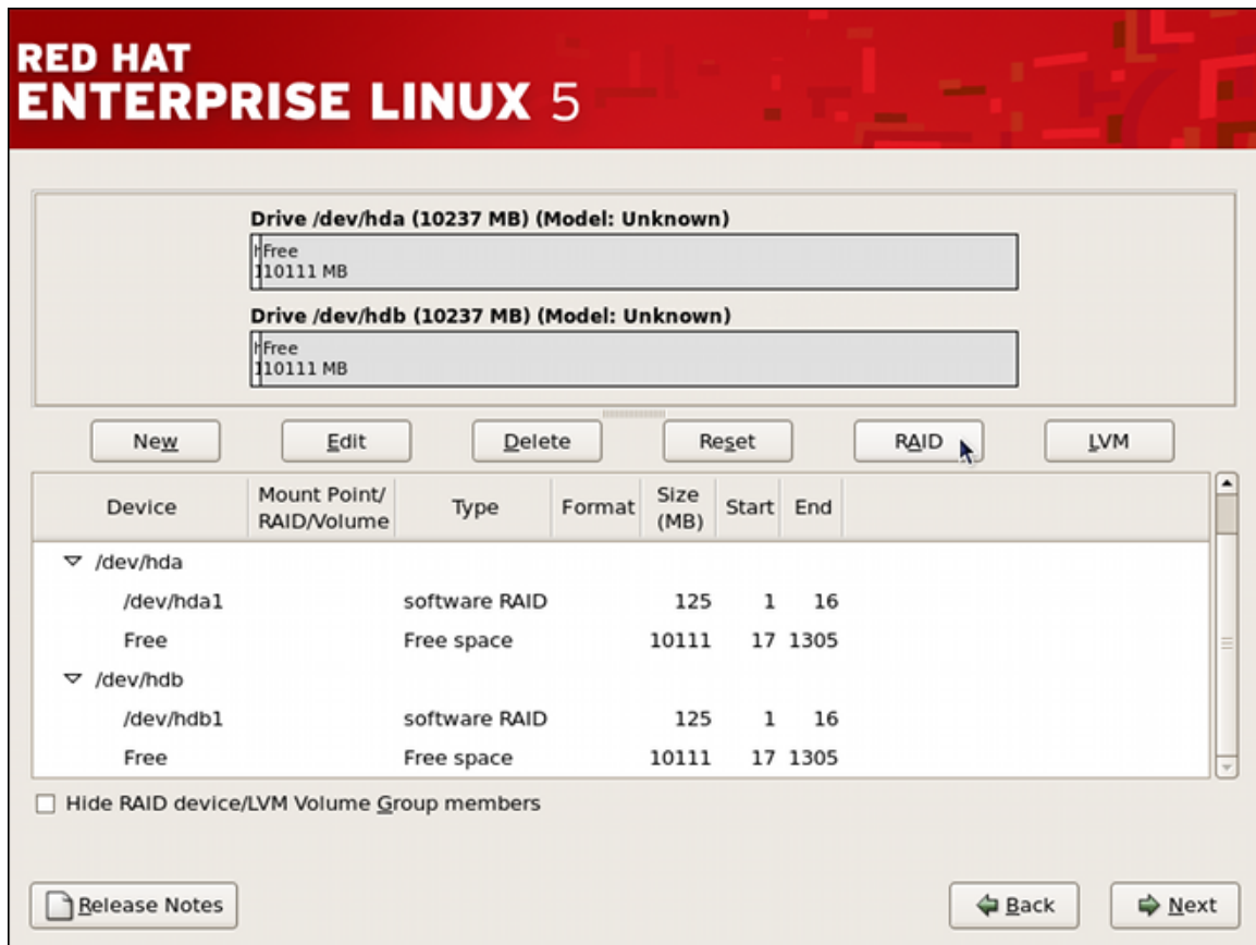
Figure 5.4. RAID 1 Partitions Ready, Pre-Device and Mount Point Creation
