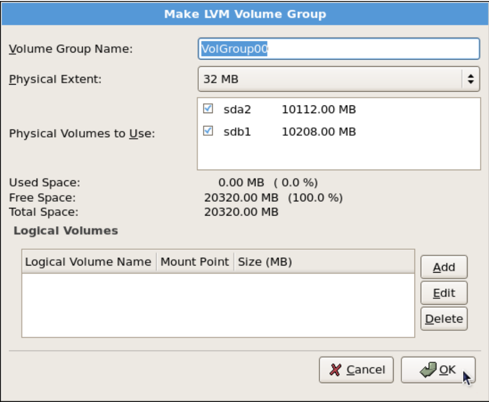
Figure 10.9. Creating an LVM Volume Group
