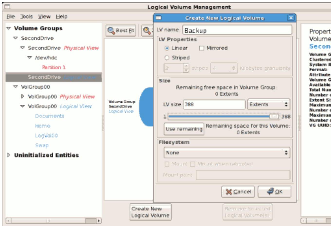
Figure 10.27. Create new logical volume
