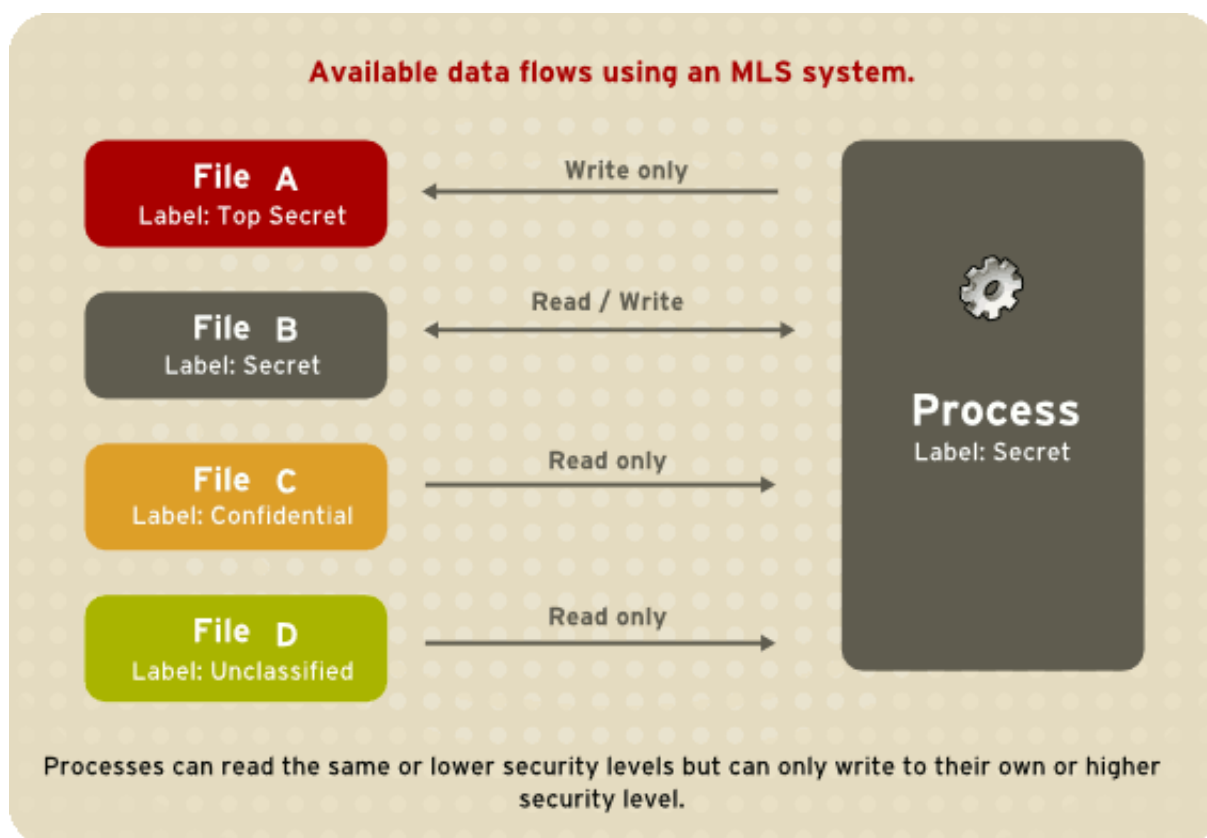
Figure 47.3. Available data flows using an MLS system
