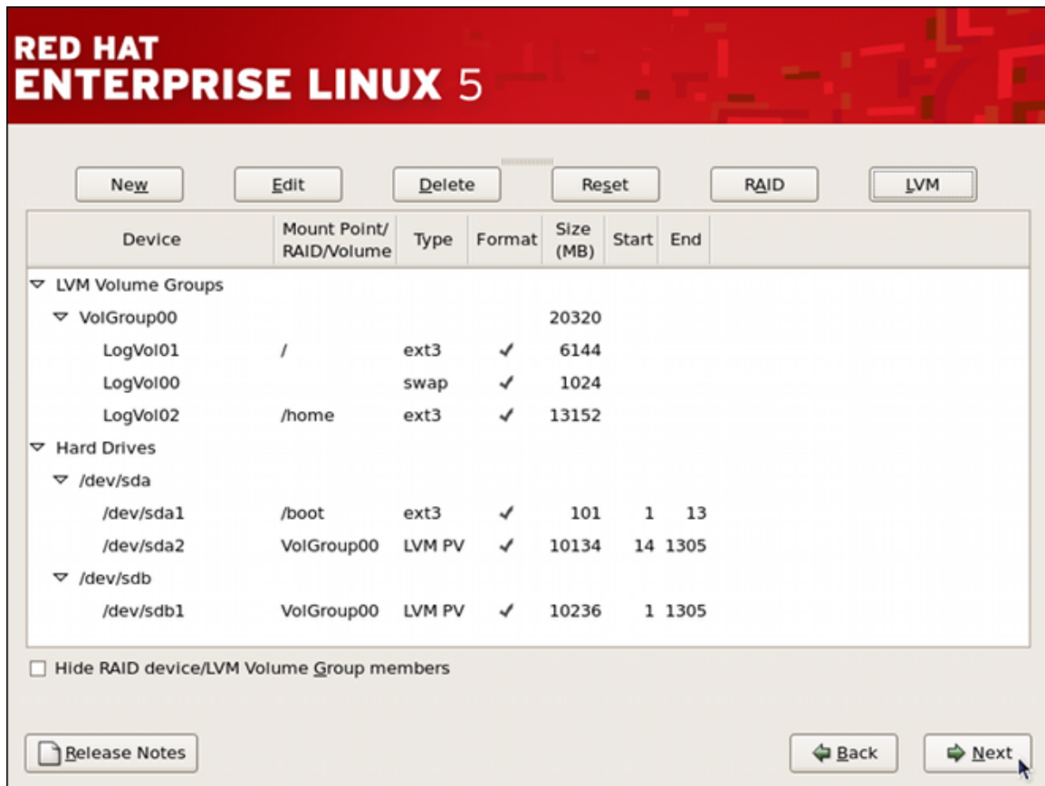
Figure 10.12. Final Manual Configuration
