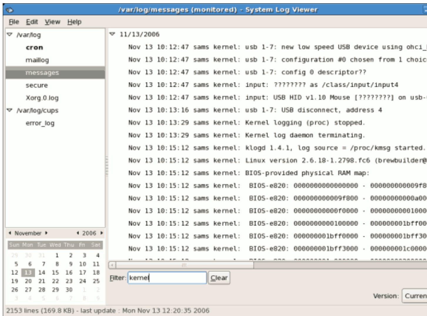
Figure 38.3. System Log Viewer - Filter
