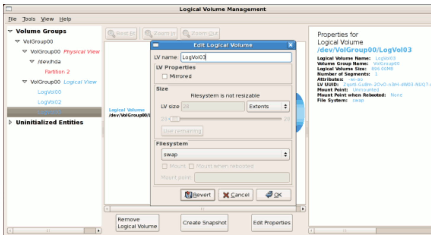
Figure 10.16. Edit Logical Volume
