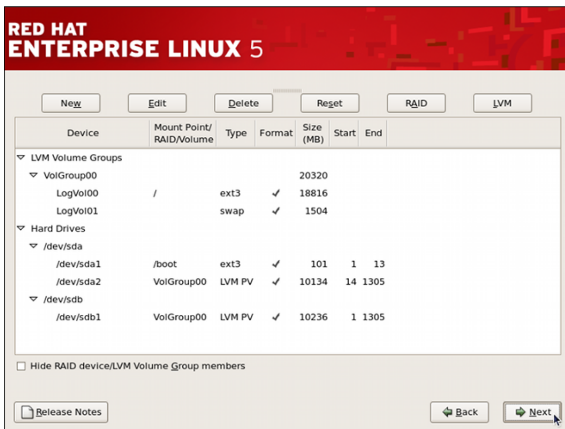
Figure 10.3. Automatic LVM Configuration With Two SCSI Drives
