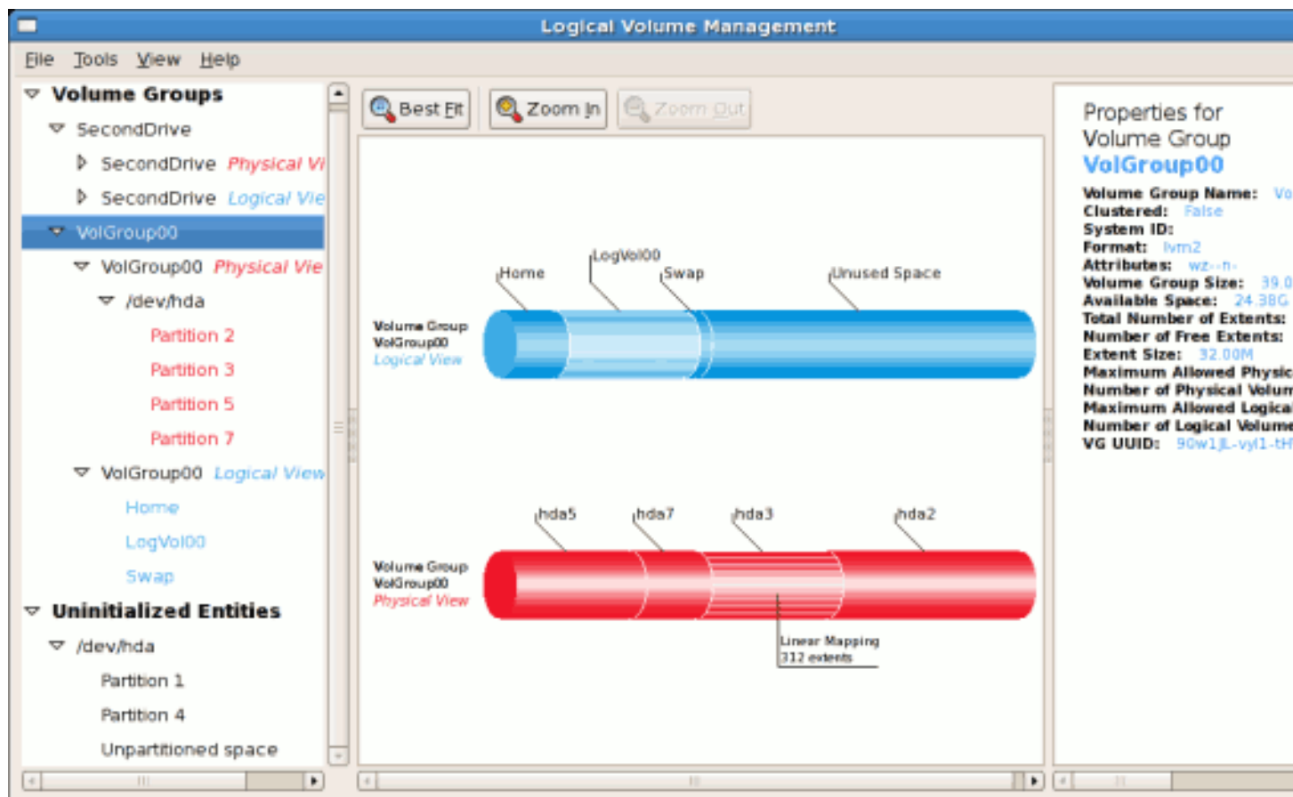
Figure 10.24. Logical and physical view of volume group
