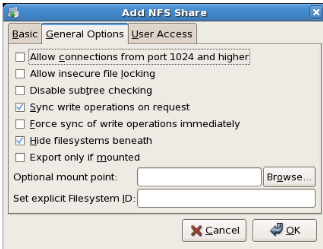
Figure 20.4. NFS General Options
