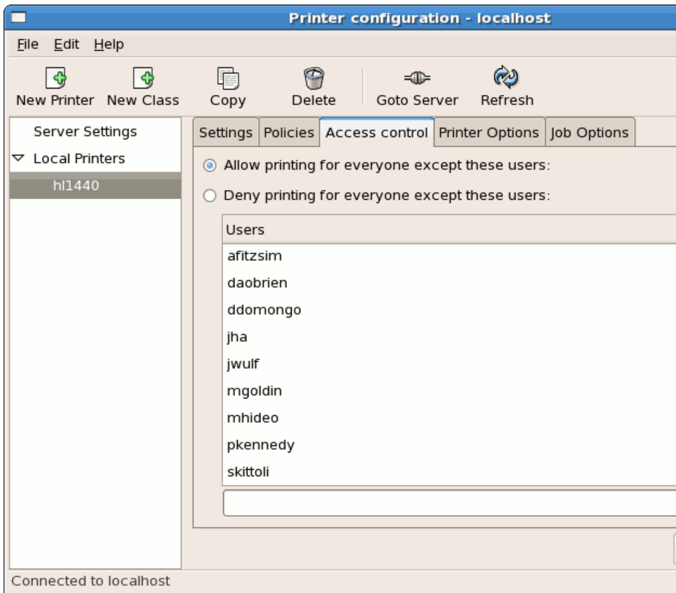
Figure 36.10. Access Control Tab
