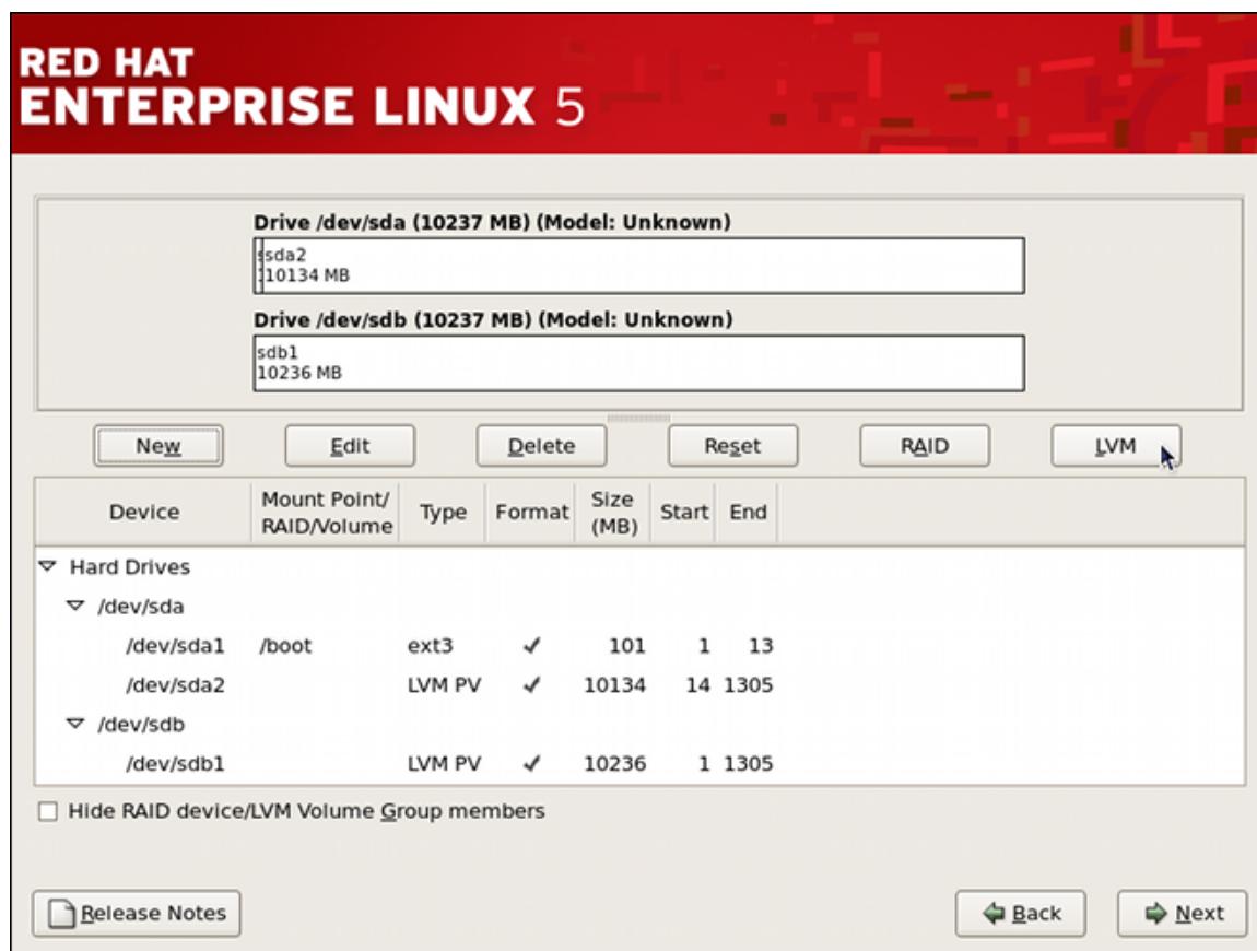
Figure 10.8. Two Physical Volumes Created
