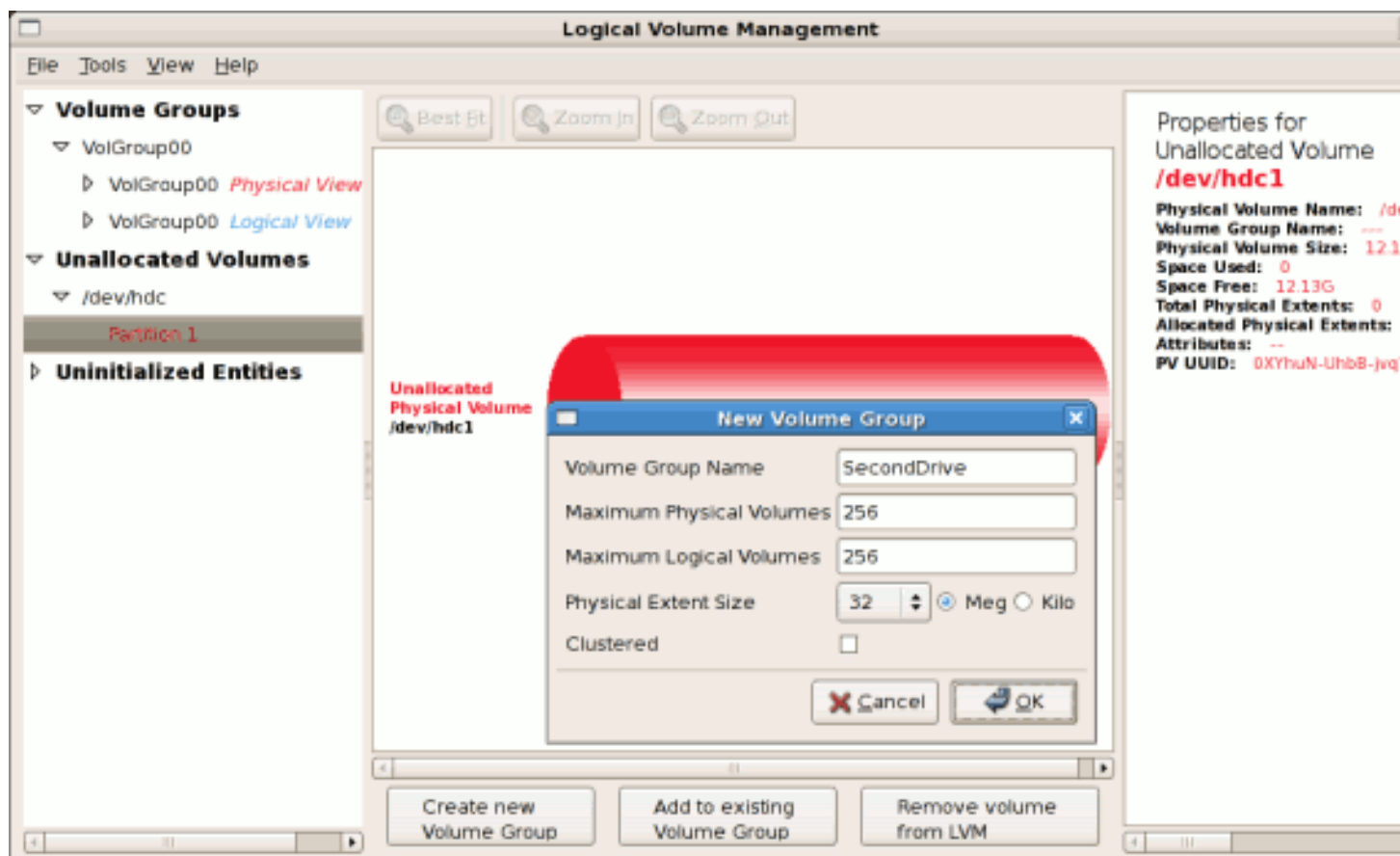
Figure 10.26. Create new volume group
