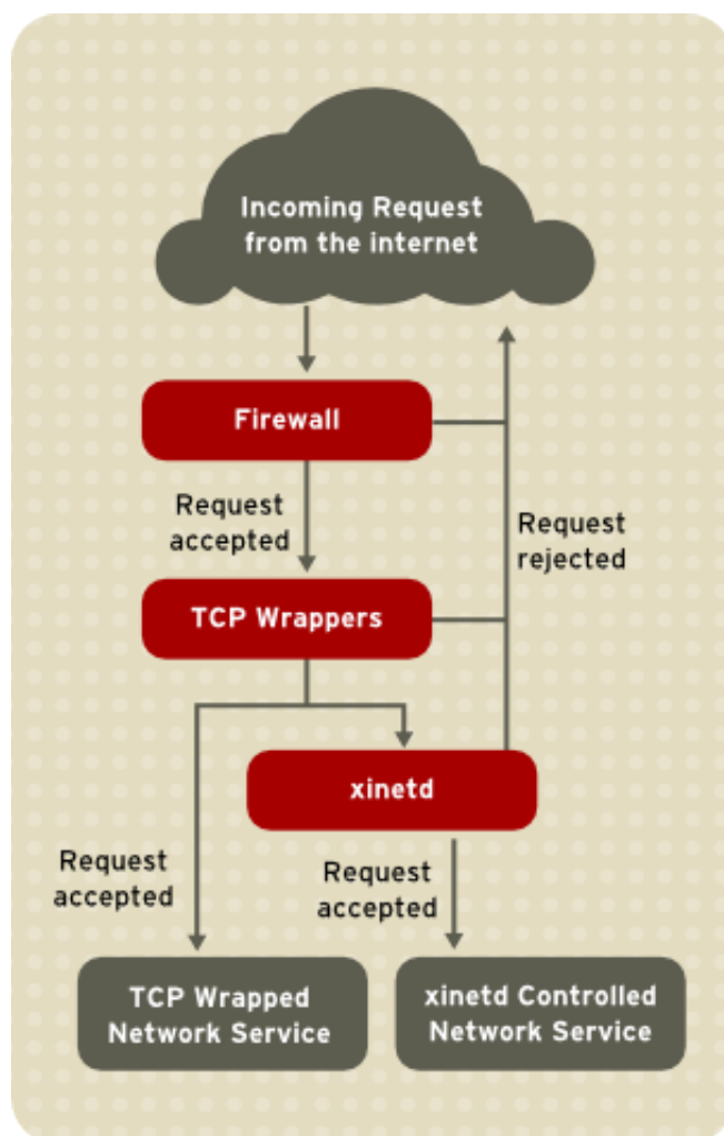
Figure 46.9. Access Control to Network Services
