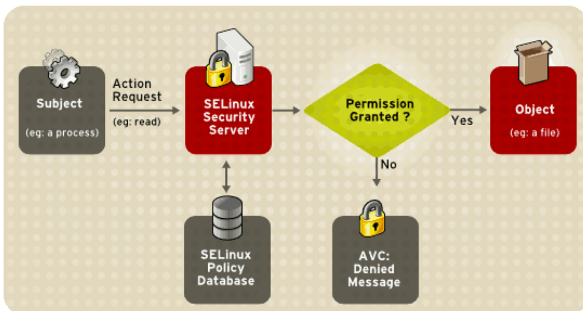
Figure 47.1. SELinux Decision Process
