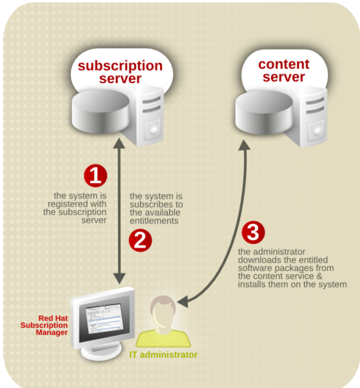
Figure 14.2. Relationship Among Systems, the Subscription Service, and Content Delivery Network
