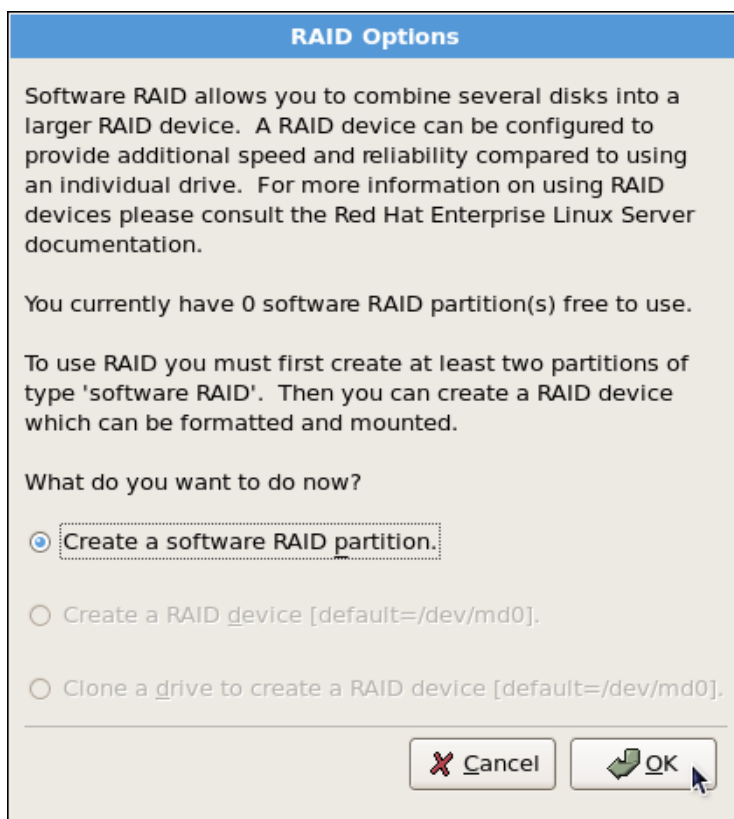
Figure 5.2. RAID Partition Options
