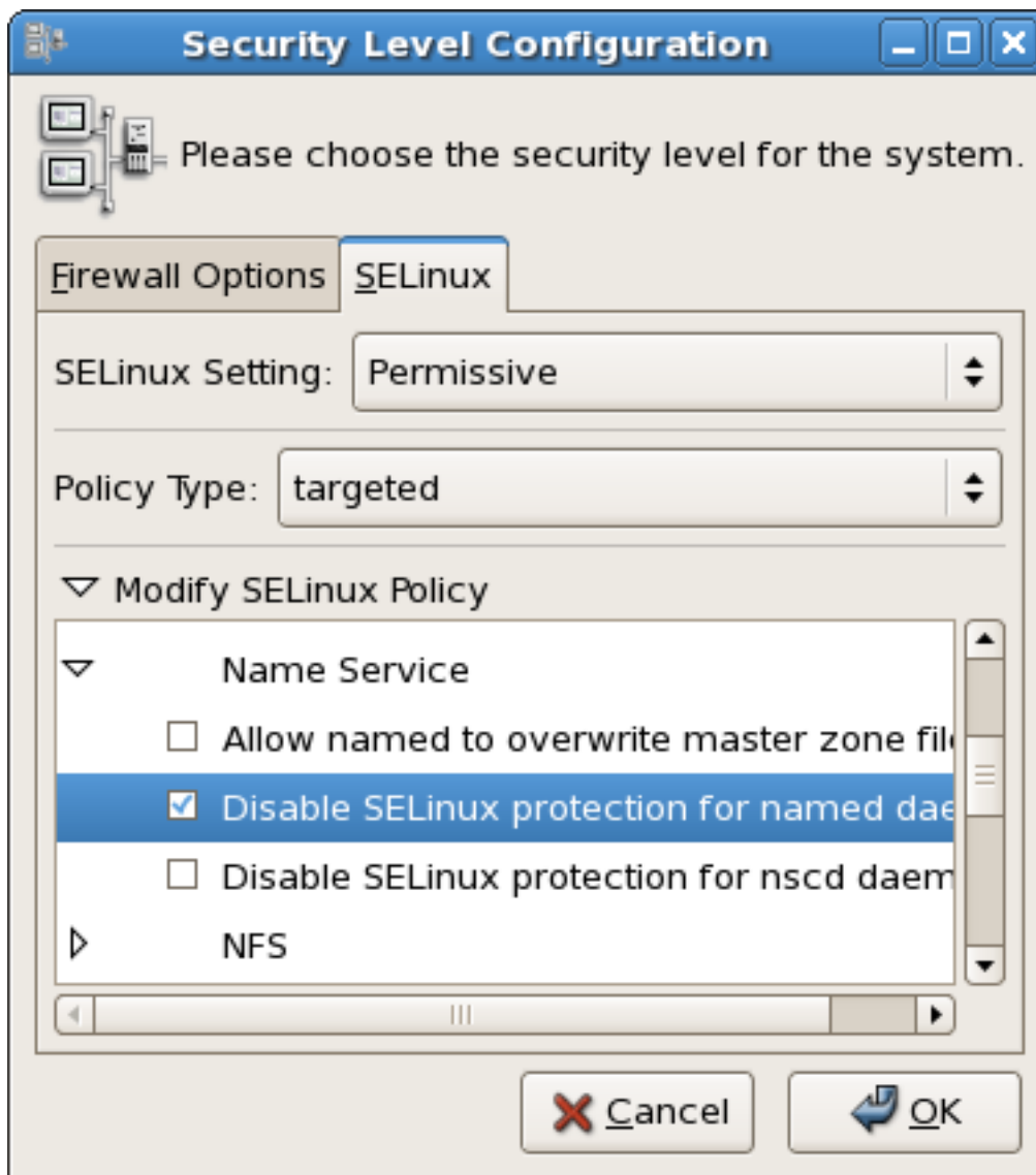
Figure 48.1. Using the Security Level Configuration dialog box to change a runtime boolean.
