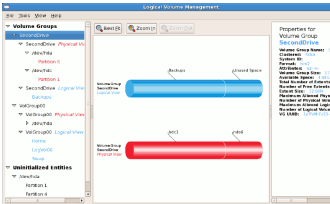
Figure 10.30. Logical and physical view of an extended volume group
