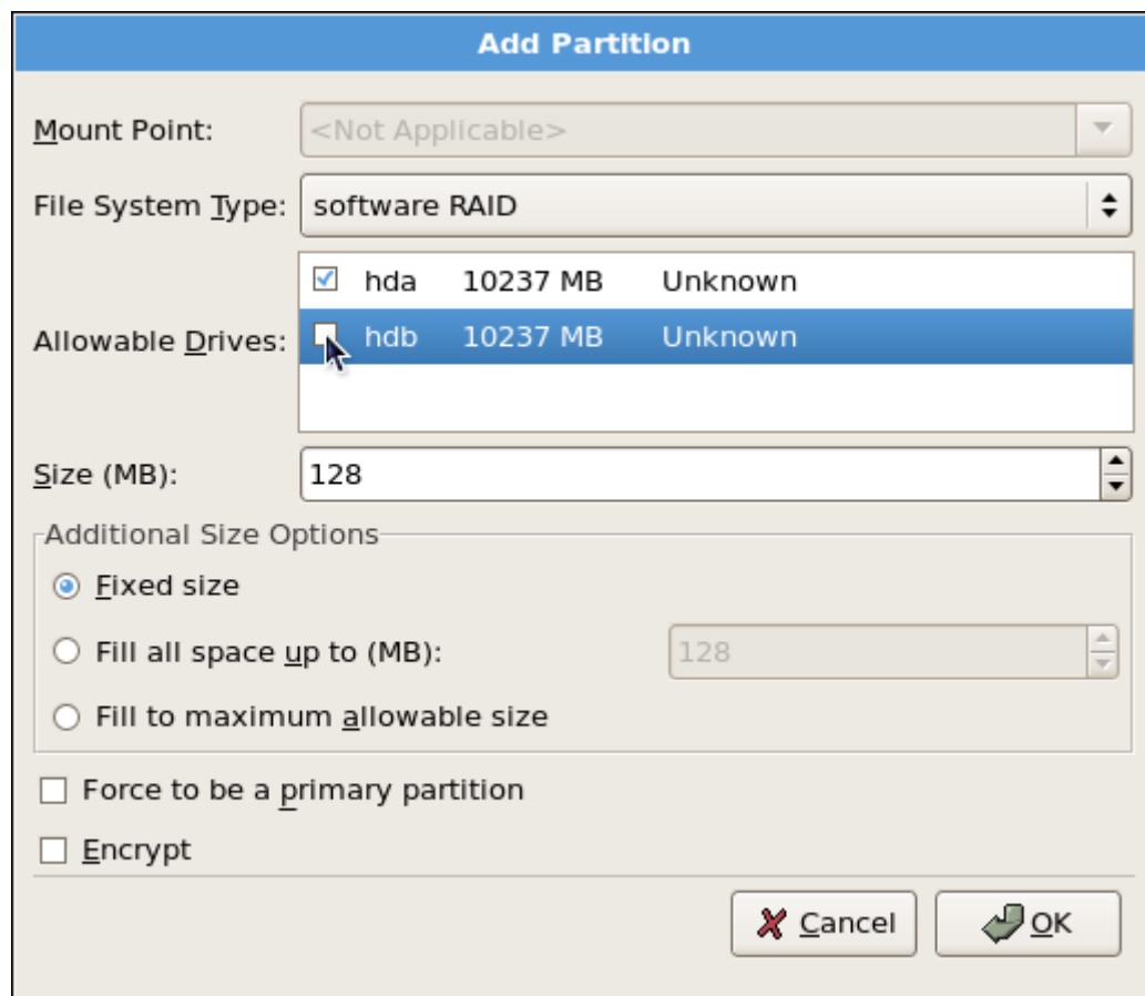
Figure 5.3. Adding a RAID Partition
