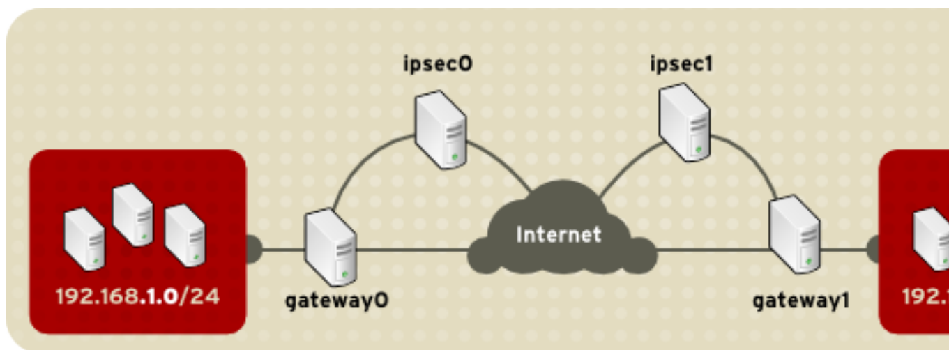
Figure 46.11. A network-to-network IPsec tunneled connection
