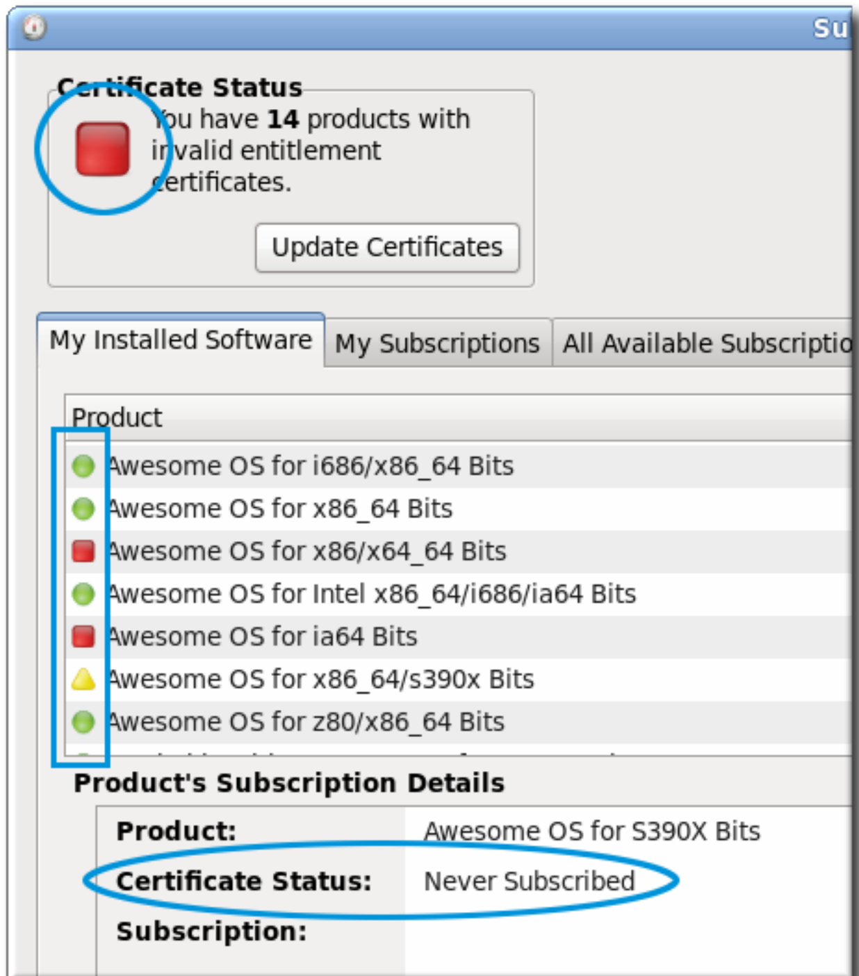
Figure 14.17. Color-Coded Status Views
