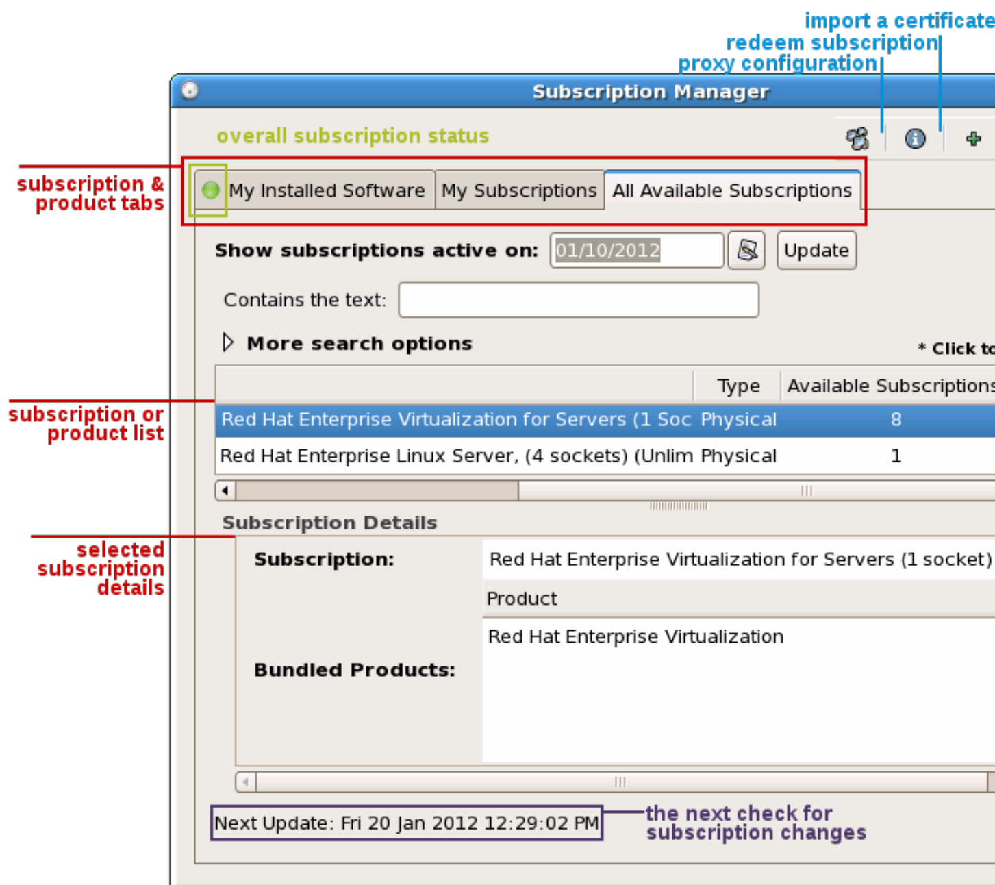
Figure 14.4. Red Hat Subscription Manager Main Screen
