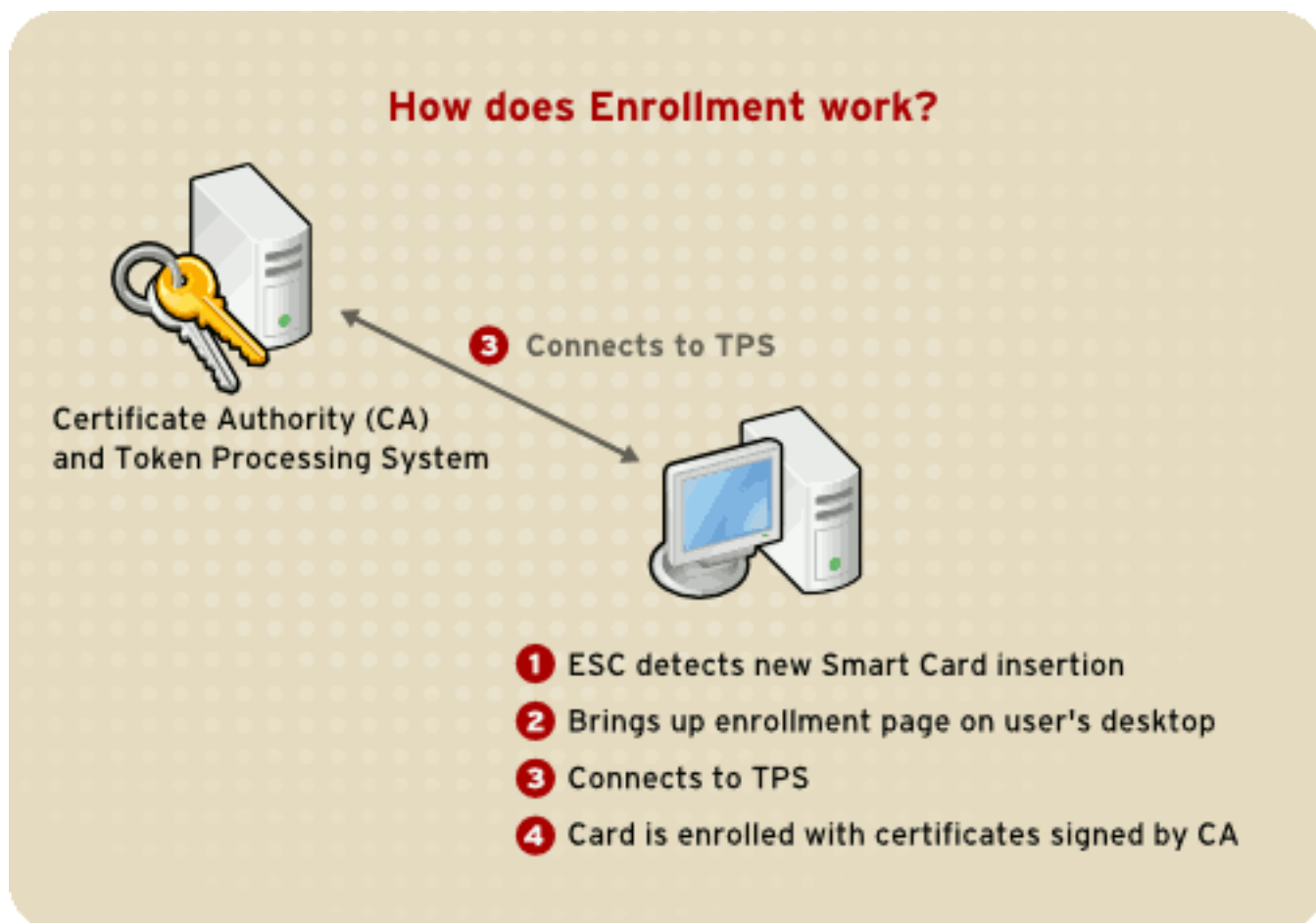
Figure 46.4. How Smart Card Enrollment Works
