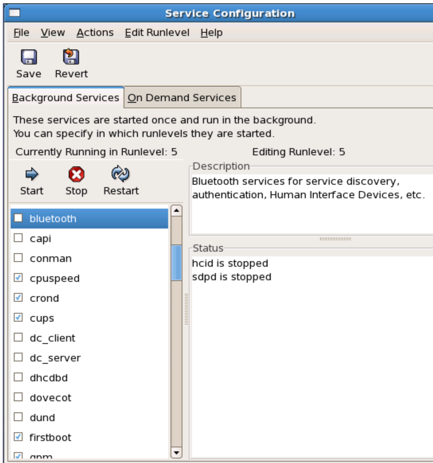
Figure 17.1. Services Configuration Tool
