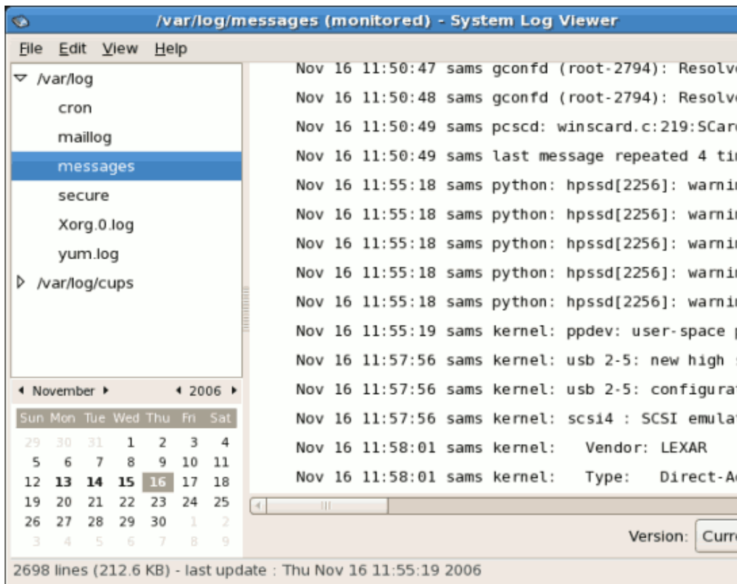
Figure 38.7. Log file contents after five seconds
