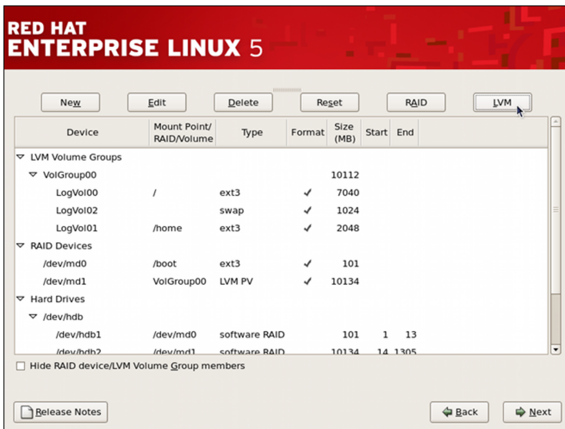
Figure 5.8. Sample RAID With LVM Configuration
