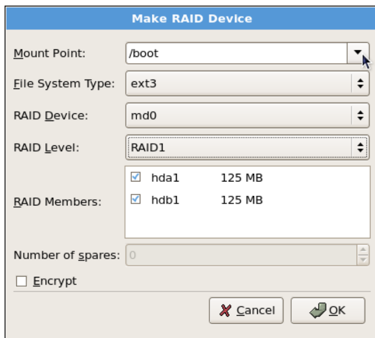
Figure 5.6. Making a RAID Device and Assigning a Mount Point
