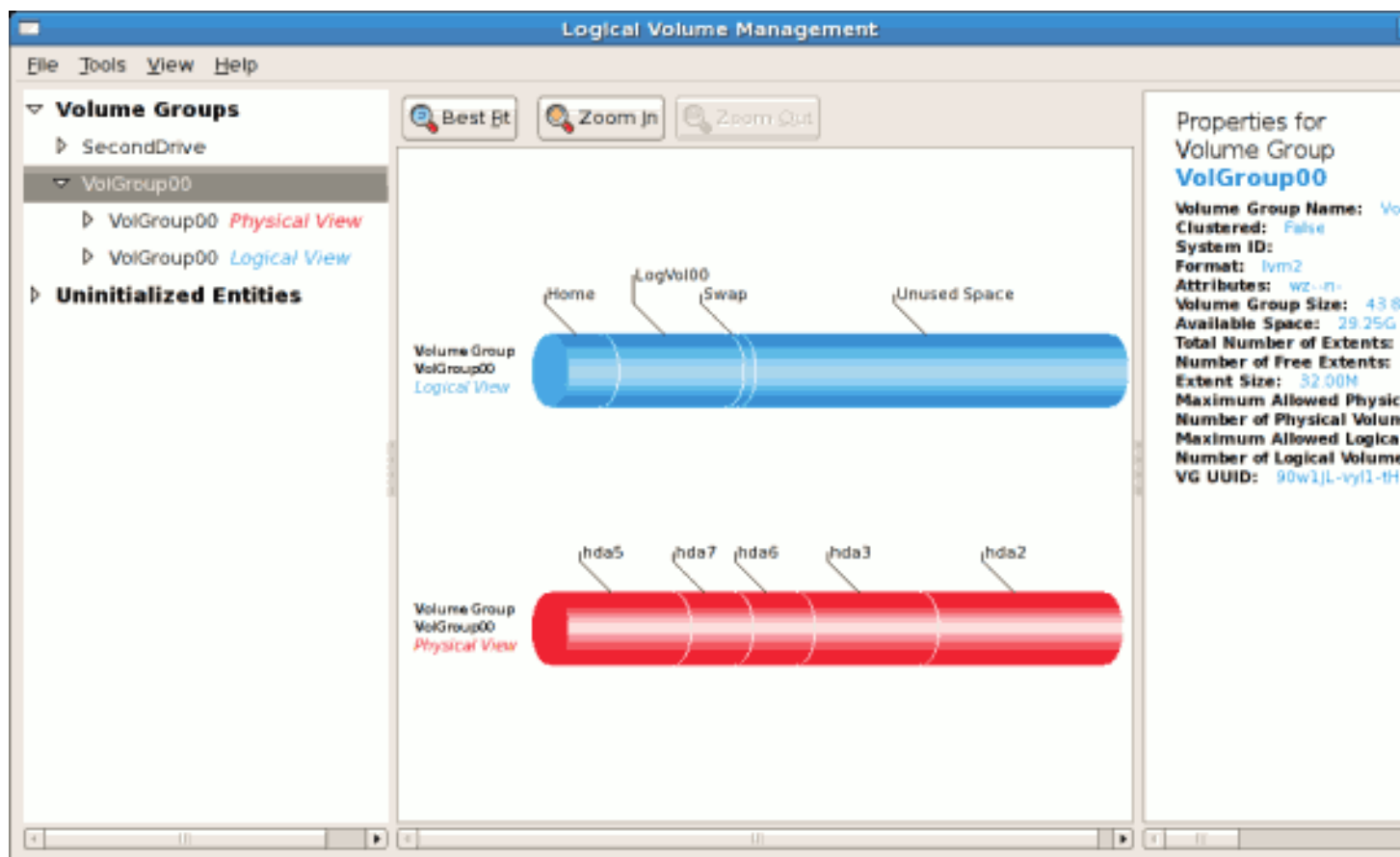
Figure 10.21. Logical view of volume group
