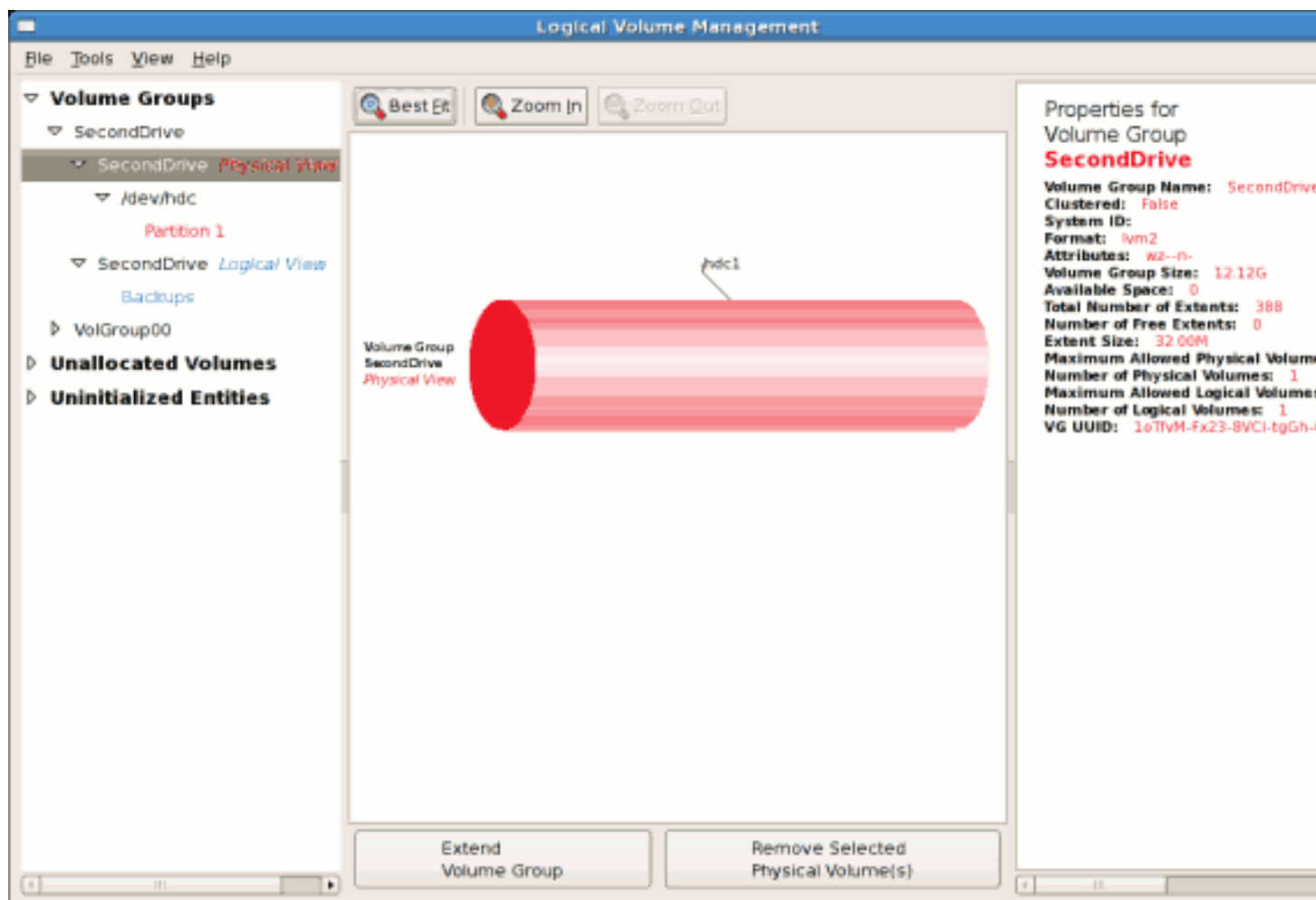
Figure 10.28. Physical view of new volume group
