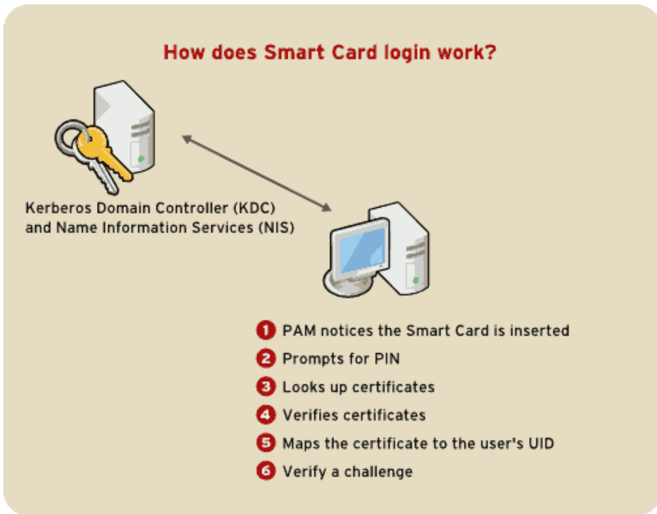
Figure 46.5. How Smart Card Login Works
