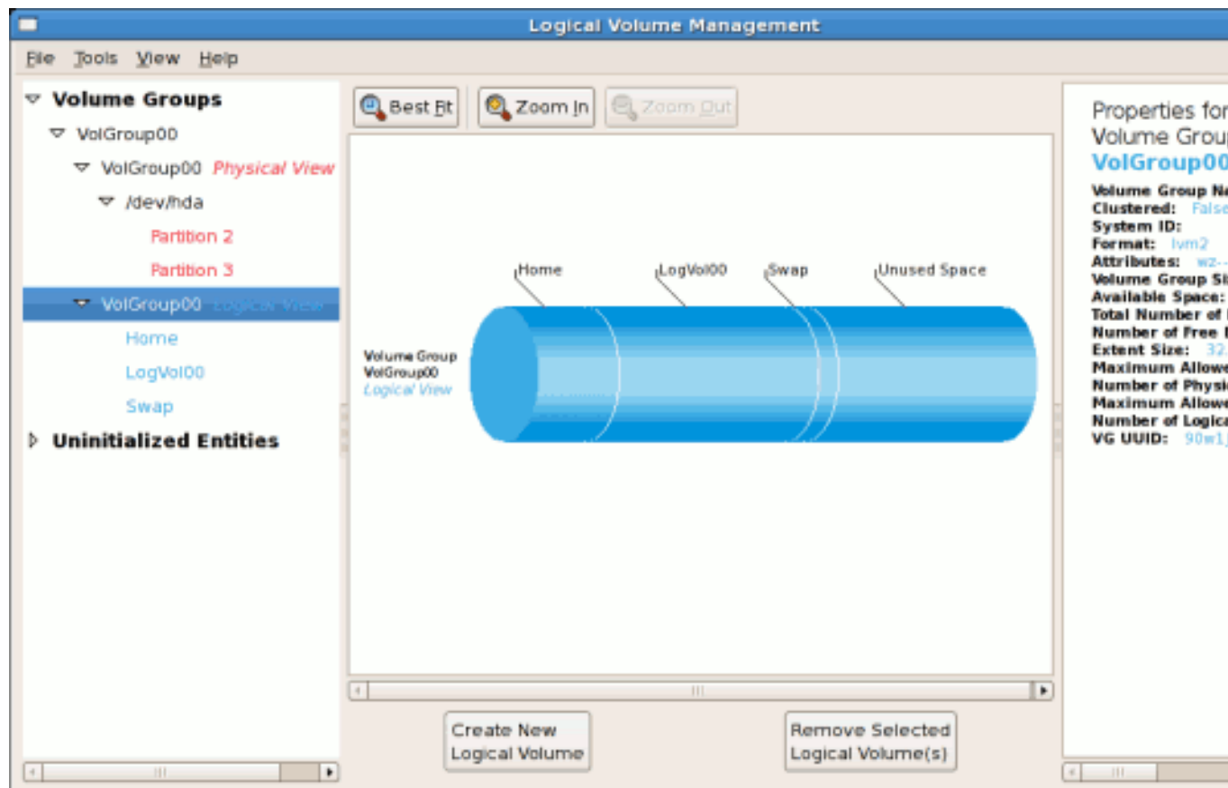
Figure 10.20. Logical view of volume group
