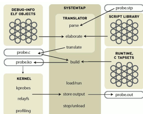
Figure 39.1. Flow of Data in SystemTap
