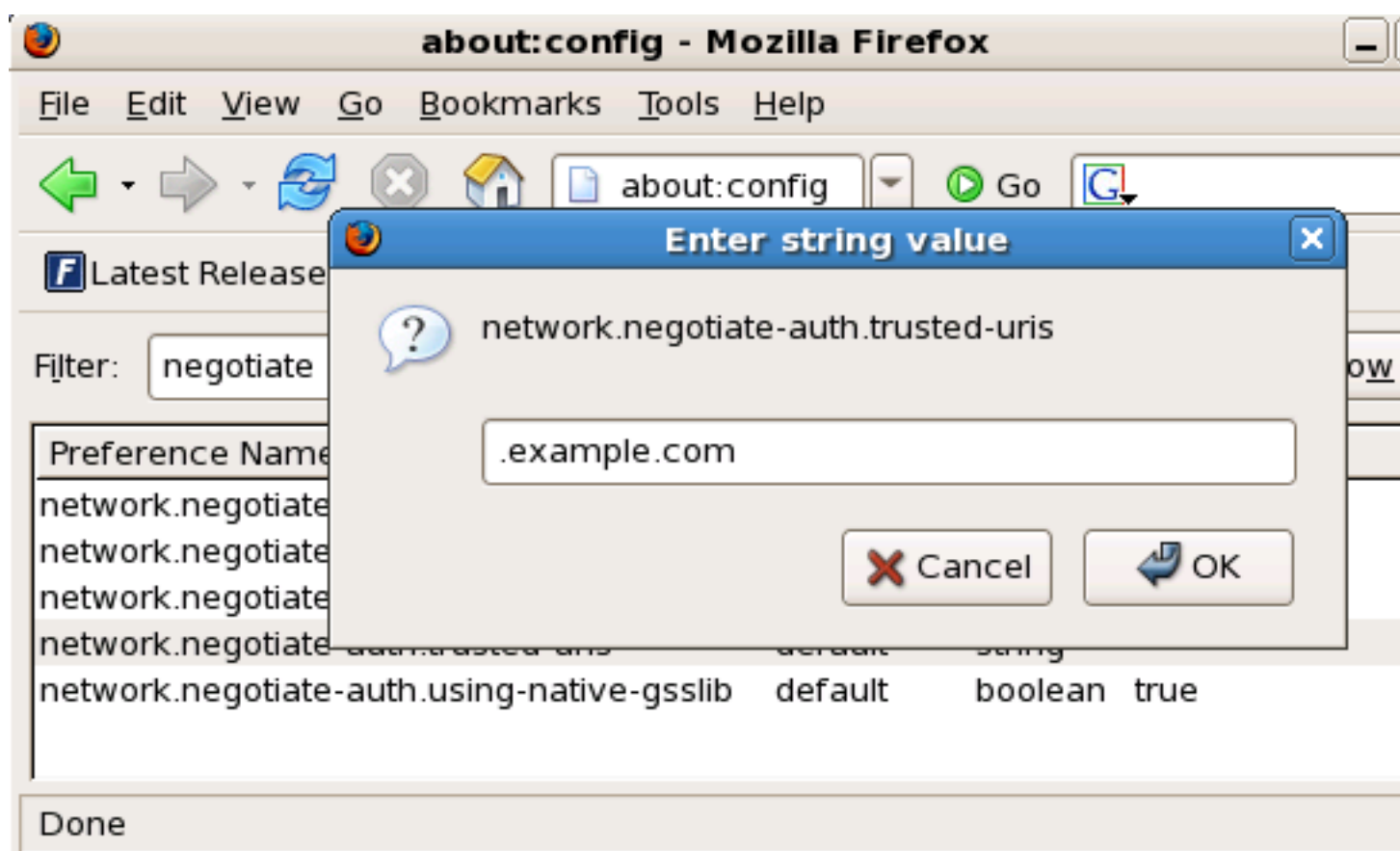
Figure 46.6. Configuring Firefox for SSO with Kerberos
